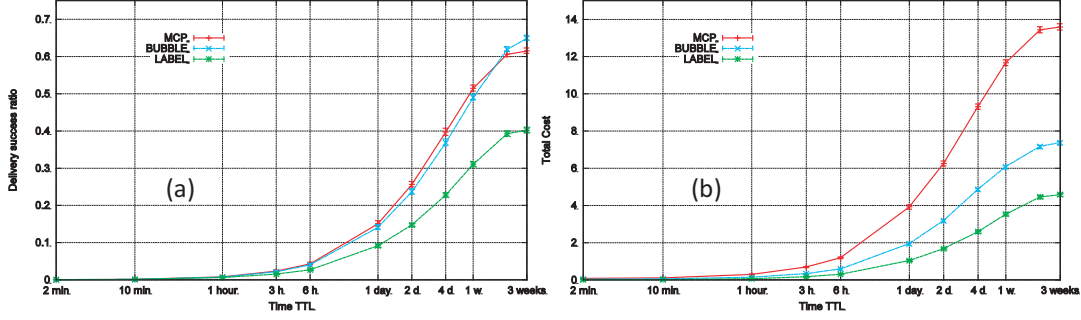
Figure 8: Comparisons of several algorithms on Reality dataset, single group.
