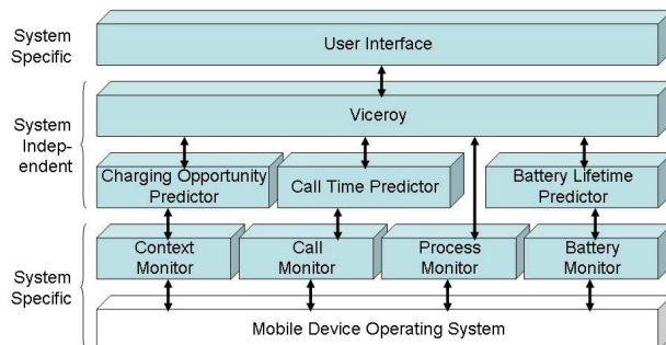
Figure 1. CABMAN system architecture
